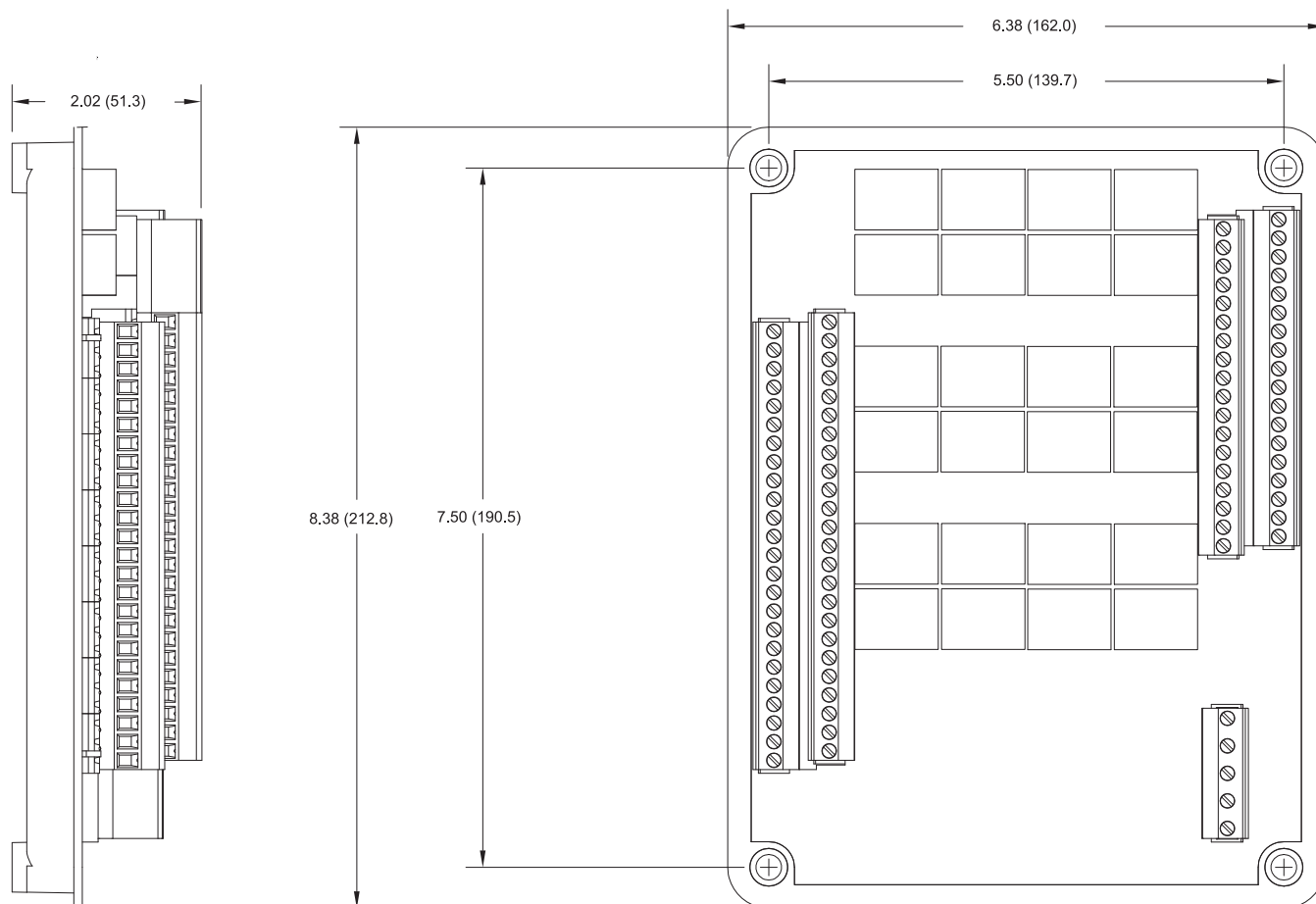
Figure 7 - CEM-2020 Overall Dimensions
